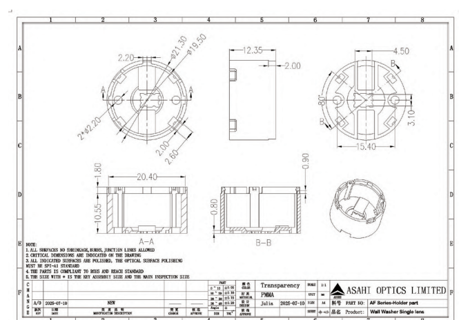
AF Series-Holder part (3535LED)
