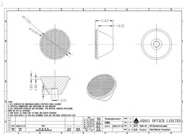
AF Series-lens part (symmetric beam)
